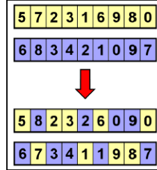
Figura 32: Uniform Crossover [21]
